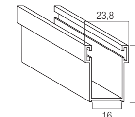
Guida in alluminio A16 GUAL..16M 16 x 28 mm
