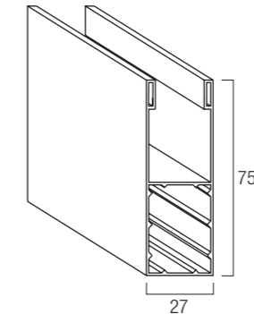
Guida in alluminio A75 GUAL..75M 27 x 75 mm
