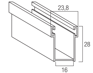
Guida in alluminio A16 GUIAL..16M 16 x 28 mm
