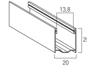
Guida in alluminio A25 GUIAL..25M 20 x 25 mm
