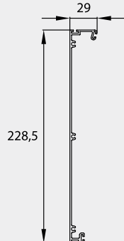
Profilo cassetto interno Internal cassette profile
