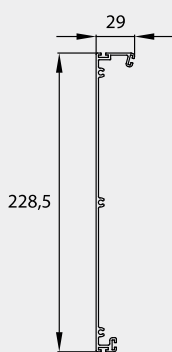
Profilo cassetto interno Internal cassette profile
