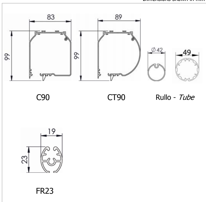
Dimensioni in mm Dimensions shown in mm
